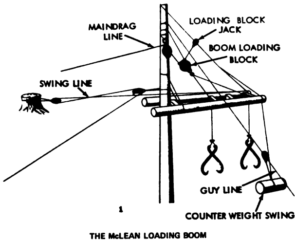
1 THE McLEAN LOADING BOOM
